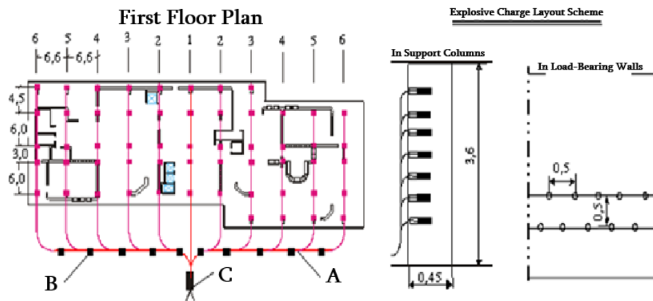
Fig. 5.9. Layout of explosive charges in supporting structures of the Batumi hotel and their slightly delayed detonation scheme:
