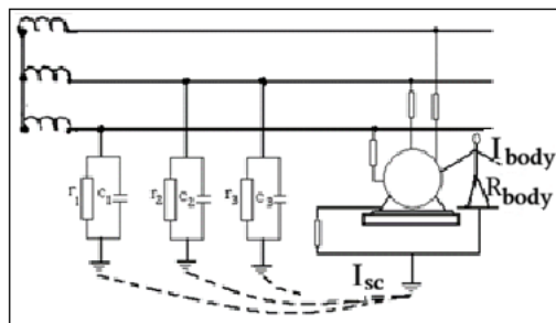
Fig. 9.14. Protective grounding scheme
