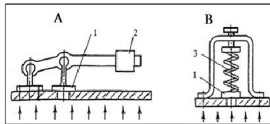
Fig. 11.5. Safety valve designs:
