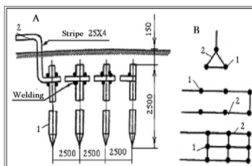
Fig. 9.18. Grounding device calculation:
