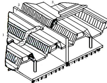
Fig. 5.4. Fire-prevention walls (grandmauers):
