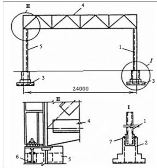
Fig. 10.8. Protection of a Category I building using metal trusses (reinforcement used as conductor and grounding):
