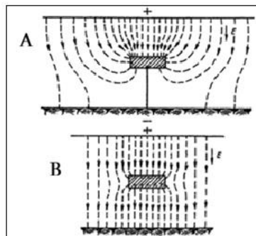
Fig. 6.1. Distortion of the Electric Field by Introducing a Grounded (A) and Ungrounded (B) Metallic Object
