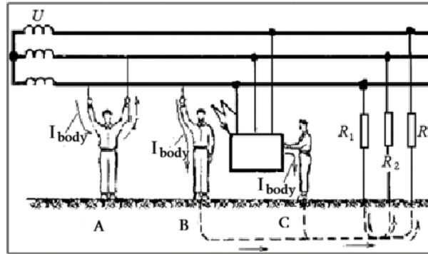
Fig. 9.12. Contact with conductors of a three-phase network: A - Two-pole contact; B, C - Single-pole contact; R_1, R_2, R_3 — total insulation resistances of conductors relative to ground
