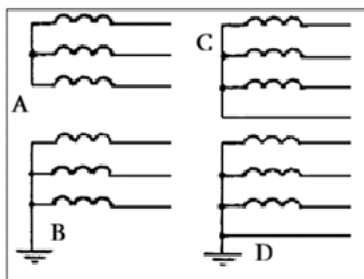
Fig. 9.11. Three-phase network schemes:
