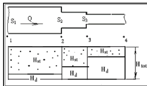
Fig. 4.4. Illustration of static and dynamic pressure variations in a variable cross-section air duct
