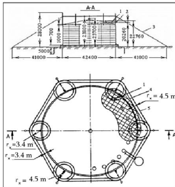
Fig. 10.9. Lightning rod for a metal reservoir with 20,000 m³ capacity:
