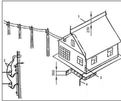
Fig. 10.10. Lightning rod for a rural house:
