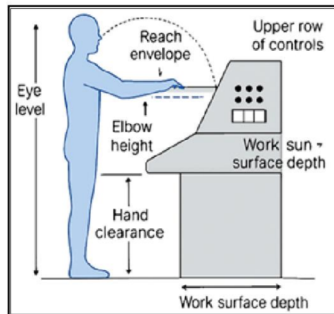
Fig. 2.10. Ergonomic arrangement of controls in a workplace. Standing posture
