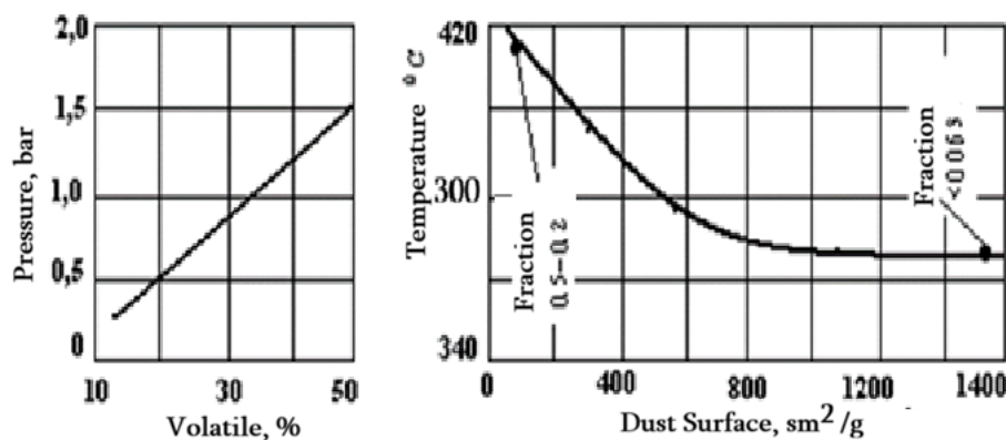
Fig. 5.1. Left — pressure development during coal dust explosion depending on volatile yield; Right — variation of ignition temperature with specific surface area
