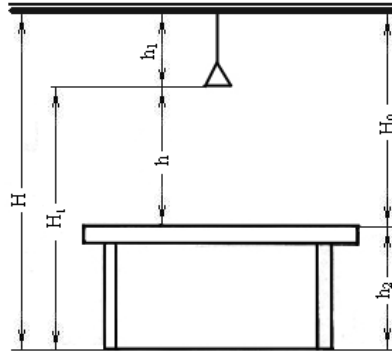
Fig. 7.3. Illustration of artificial lighting
