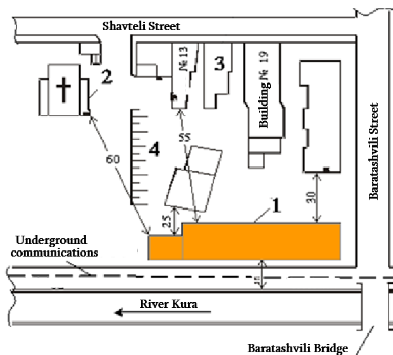
Fig. 5.7. Situational plan of the knitwear factory and protected objects: 1 – Knitwear factory building; 2 – Anchiskhati Church (6th century); 3 – Residential brick houses built in the 19th and early 20th centuries; 4 – Locations of seismic receivers
