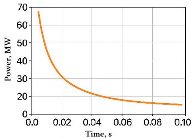
Fig. 11.3. Variation of explosion power over time
