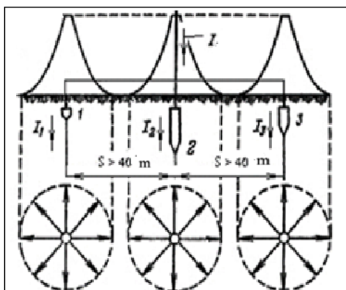
Fig. 9.5. Curves of potential and current dispersion fields of a group grounding device, when the distance between electrodes is greater than 40 m. Group grounding electrodes
