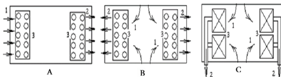
Figure 4.11. Ventilation Schemes of Premises:
