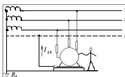
Fig. 9.19. Neutralization scheme
