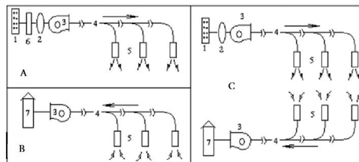
Fig. 4.13. Illustration of General and Local Ventilation Systems:
