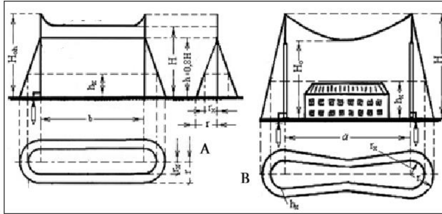
Fig. 10.4. Schemes of protection zone calculation parameters for lightning rods: A – wire-type lightning rod; B – double rod-type lightning rod of equal height
