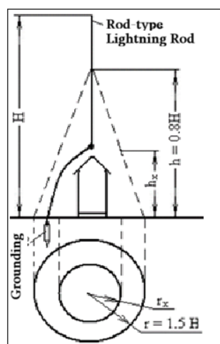
Fig. 10.3. Calculation parameters of the protection zone of a single rod-type lightning rod
