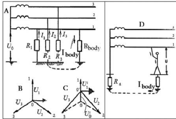
Fig. 9.13. Single-pole contact illustration in three-phase grounded-neutral (a, b, c) and isolated-neutral unexpended (D) networks
