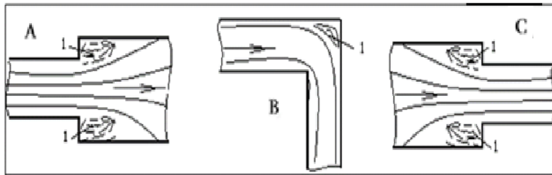
Fig. 4.6. Illustration types of local resistances:
