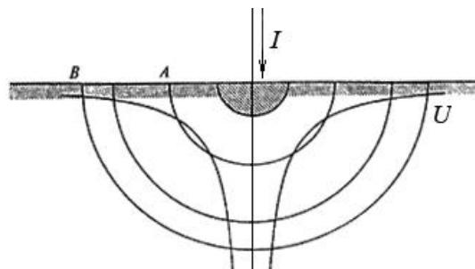
Fig. 9.8. Scheme of current flow into the ground during a short circuit
