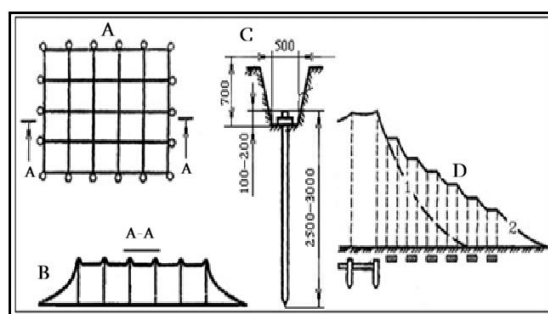
Fig. 9.17. Calculation of grounding devices:
