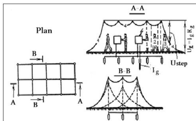
Fig. 9.16. Contour grounding device:
