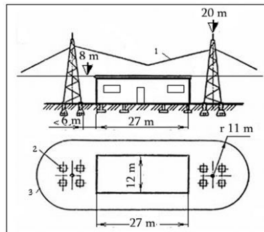
Fig. 10.6. Protection of a Category I building with a separate double rod-type lightning rod (soil resistivity 300 \Omega \cdot \text{m} ):
