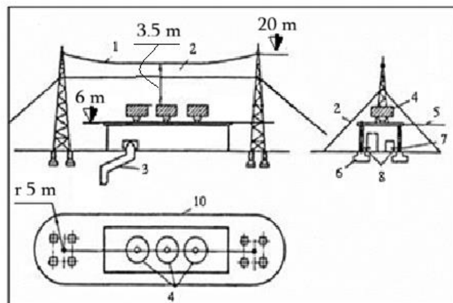
Fig. 10.7. Protection of a Category I building with a separate wire-type lightning rod (soil resistivity 300 \Omega \cdot \text{m} ):
