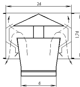
Fig. 4.15. Deflector:
