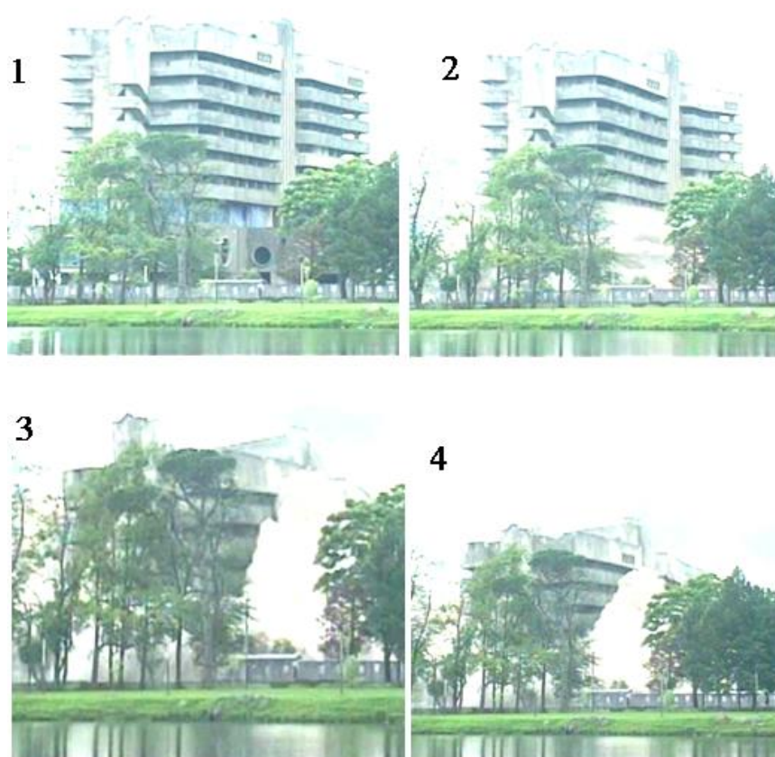
Fig. 5.10. Fragments of the demolition of the Batumi Hotel building by explosion
