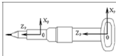
Fig. 8.7. Axes of Vibration Transmission During Local Vibration at Tool Grip Points
