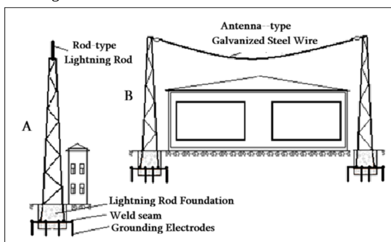
Fig. 10.1. Principle of lightning rod construction:
