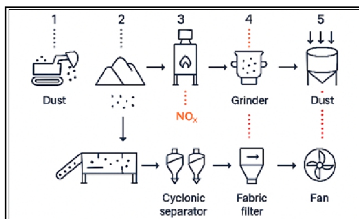
Fig. 12.1. Cement production process flow (raw material → clinker → cooling → grinding → storage)
