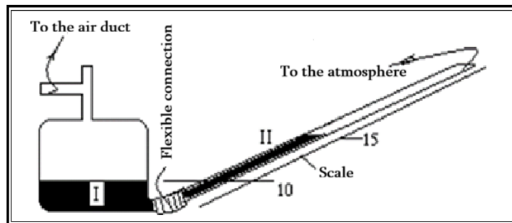
Fig. 4.3. Principle diagram of a micromanometer: I - vertical tube with a diameter of 70 mm; II - inclined tube with a diameter of 2 mm
