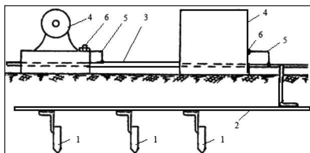
Fig. 9.15. Grounding arrangement:
