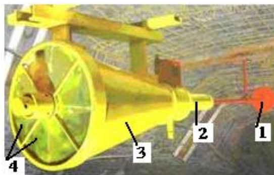
Fig. 5.2: General view of an automatic inert dust dispersion system: 1 — sensors and control panel; 2 — compressed air reservoir; 3 — container of inert dust; 4 — nozzles, normally sealed hermetically
