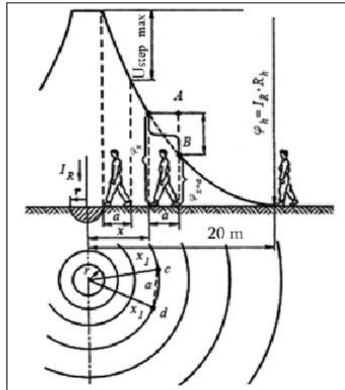
Fig. 9.9. Step voltage in the case of a single grounding electrode
