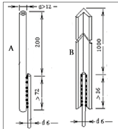
Fig. 10.2. Rod-type lightning receptor: A – made of pipe; B – made of angle bar
