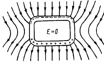
Fig. 6.2. Electrostatic Shield
