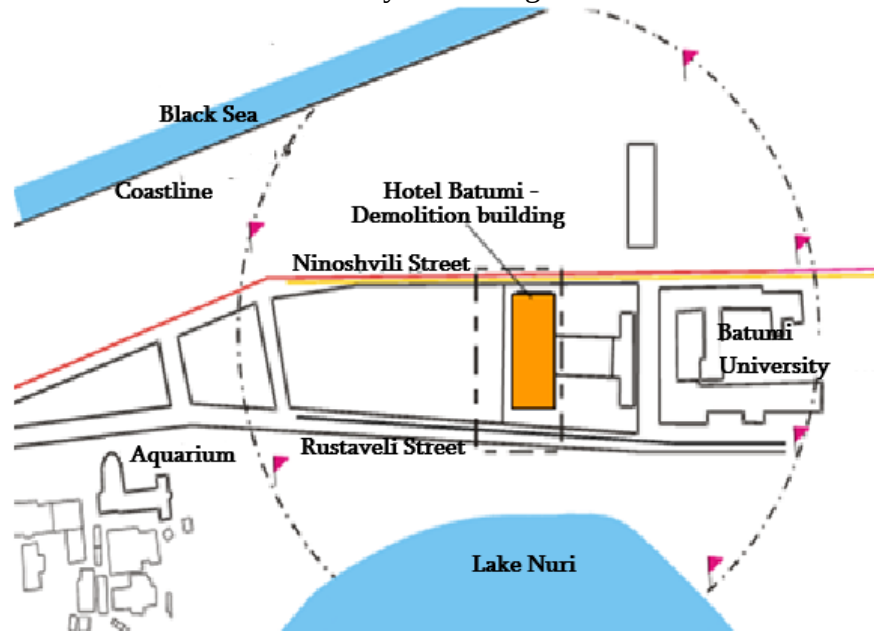
Fig. 5.8. Situational plan for the demolition of the Batumi Hotel building by explosion
