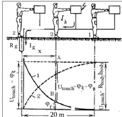
Fig. 9.7. Touch voltage for a single grounding electrode:
