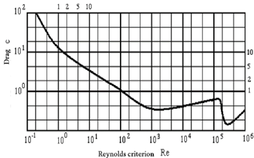
Fig. 4.10. Variation of Dimensionless Frontal Resistance Coefficient with Reynolds Number: Scale divisions shown in the range 1–10 apply equally to other ranges
