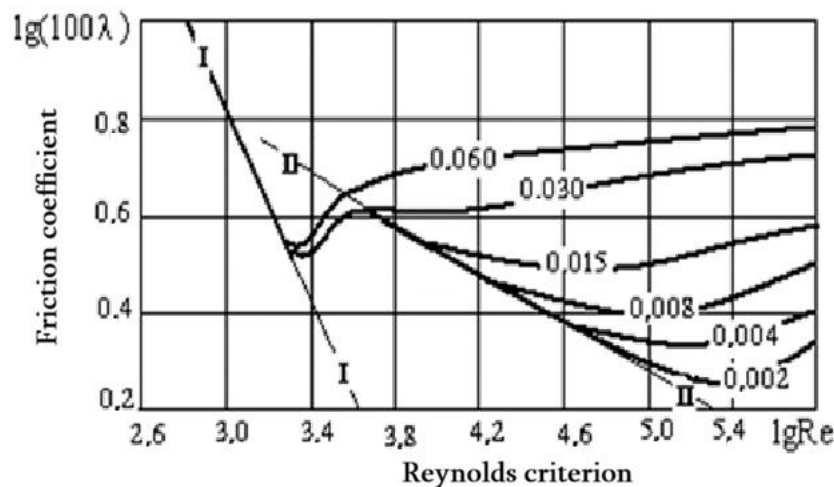
Fig. 4.8. Variation of the Dimensionless Friction Coefficient According to Flow Regime: Values such as 0.002, 0.004, etc. represent roughness calibration — the ratio of wall roughness protrusion to duct hydraulic diameter
