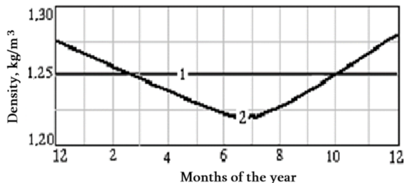
Figure 4.1. Character of Average Air Density Variation: 1 – Underground structure; 2 – Open atmosphere.
