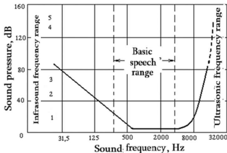
Figure 8.3. Auditory Range (according to Bell):
