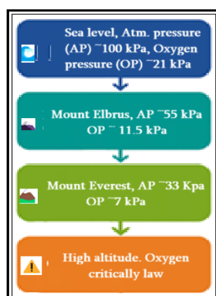
Fig. 3.1. Variation of atmospheric pressure and oxygen partial pressure: 1 – Air pressure; 2 – Oxygen partial pressure. Average values corresponding to the altitudes of Elbrus and Everest are indicated
