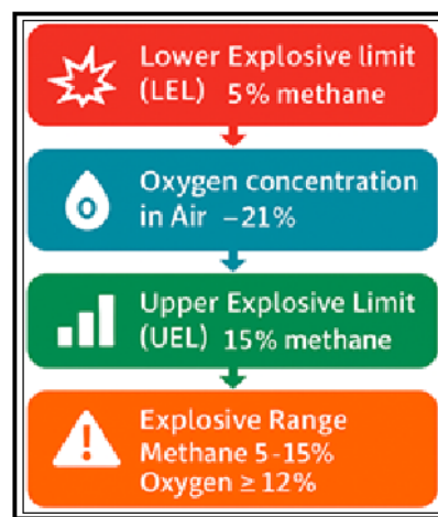
Fig. 3.5. Limits of methane explosiveness in air with oxygen
