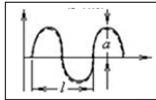
Figure 8.1. Sound wave: a – amplitude; \ell - wavelength
