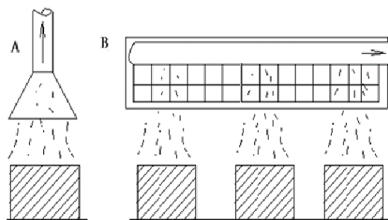
Fig. 4.16. Exhaust Hoods: A – individual; B – group (with glazed frames)
