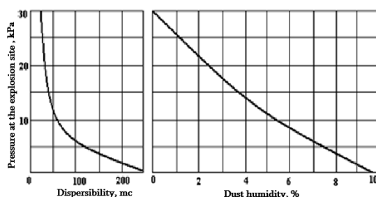
Fig. 5.3. Left – dependence of sulfur dust explosion pressure on its dispersion; Right – dependence of the same parameter on dust moisture
