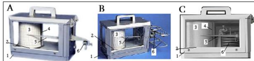
Fig. 3.14. Thermograph, Hygrograph, and Barograph:
