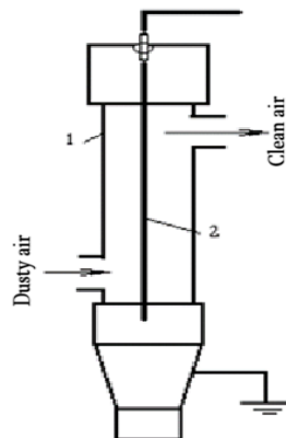
Figure 4.18. Principle Scheme of Electro filter: 1 – casing; 2 – electrode
