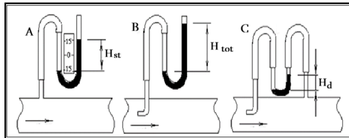
Fig. 4.2. Determination of static, dynamic and total pressure in an air duct
