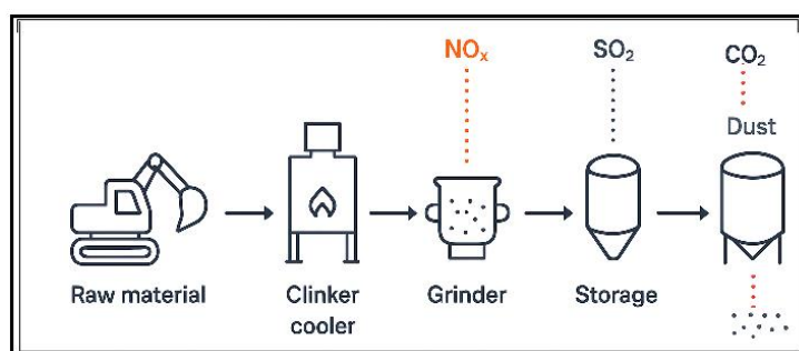
Fig. 12.2. Sources of Atmospheric Emissions and Control Mechanisms
