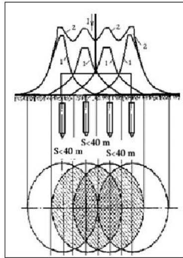
Fig. 9.6. Curves of potential and current dispersion fields of a group grounding device, when the distance between electrodes is less than 40 m: 1-Curves of the individual electrode's own potential; 2-Curves of the total potential
