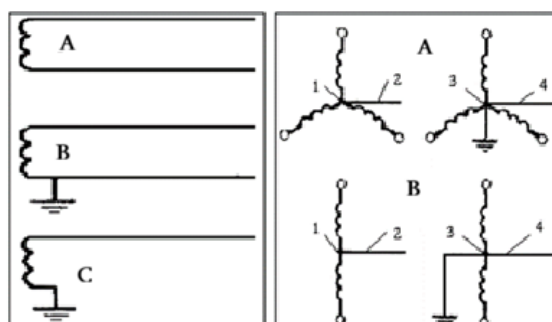
Fig. 9.10. Single-phase networks:
