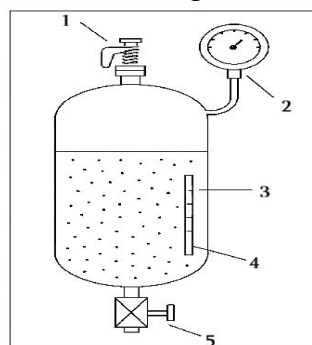
Fig. 11.2. Arrangement of safety devices on a high-pressure vessel:
