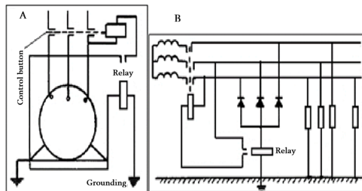
Fig. 9.20. Protective disconnection schemes:
