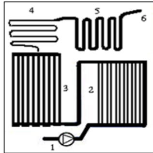
Fig. 11.8. Water and steam circulation in a direct-fired boiler:
