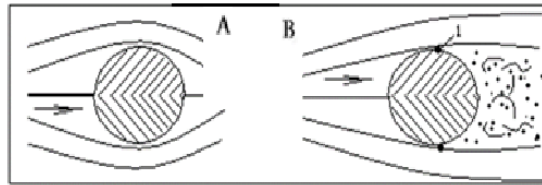
Figure 4.9. Illustration of Frontal Resistance: A – Laminar flow; B – Turbulent flow; 1 – Point of flow separation. Arrows indicate flow direction
